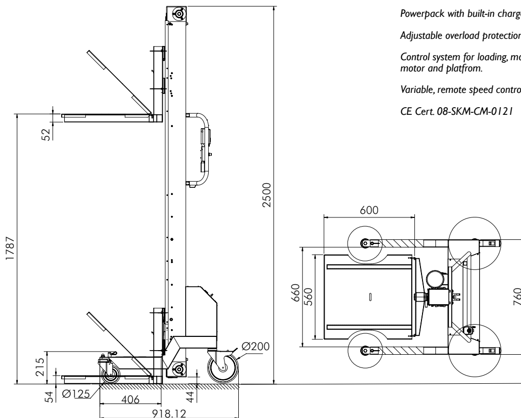
PRO200 with platform 8557, fold-up with forks
